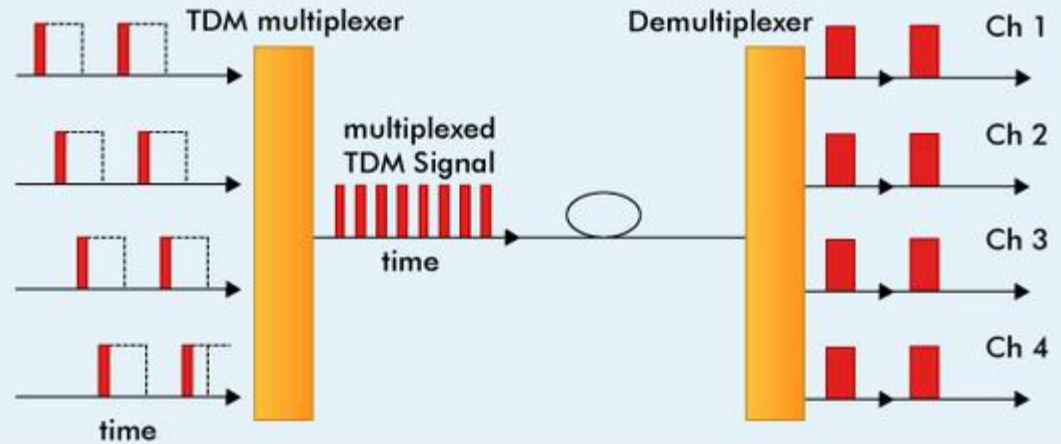
TDM (Time Division Multiplexing)
