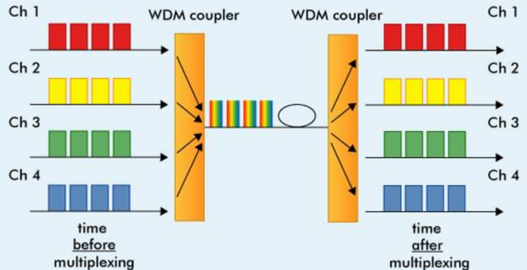
WDM (Wavelength Division Multiplexing)
